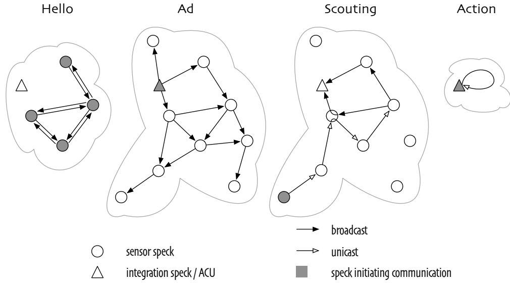
FIGURE 6.5: Illustration of messages communicated within the monitoring system, as implemented in SpeckSim. Four types of radio messages are used: Hello , Ad , Scouting and Action . For a summary, see section 6.3.2.3.
