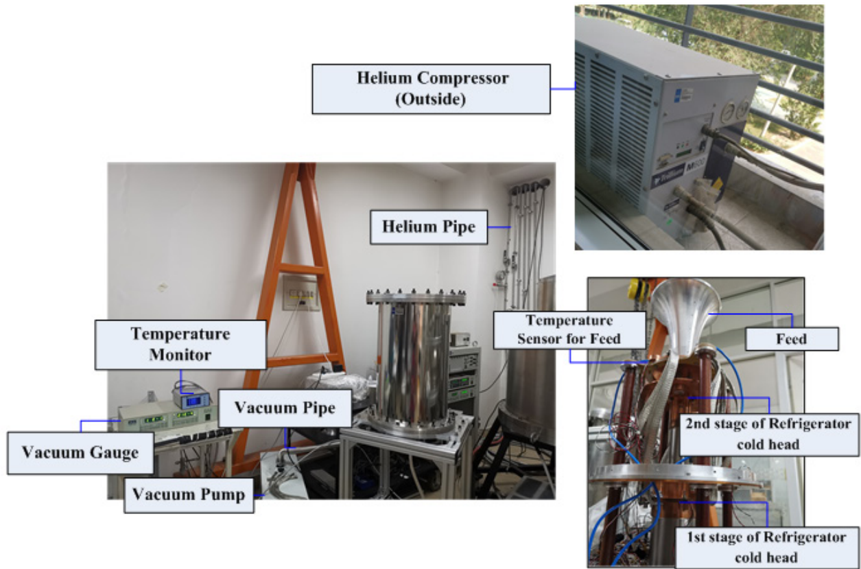
FIGURE 16. Measurement set up for Cryogenic QRHF
