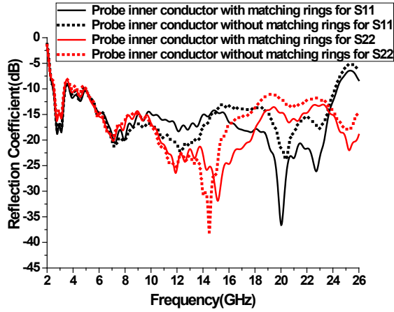
FIGURE 5. Matching rings for probe inner conductor effects on reflection coefficient
