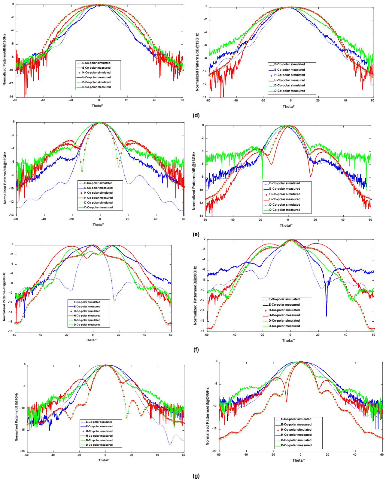
FIGURE 11. Comparisons between simulated and measured radiation pattern for (a) 2.4 GHz, (b) 4 GHz, (c) 8 GHz, (d) 12 GHz, (e) 16 GHz, (f) 20 GHz, and (g) 24 GHz, where left: Port 1 and right: Port 2.
