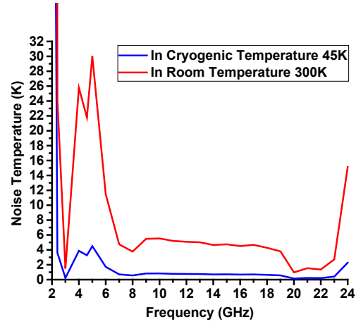
FIGURE 20. The calculated QRFH Noise contribution in different frequency bands
