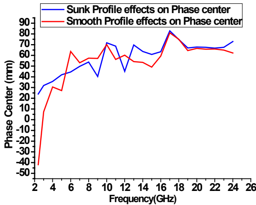
FIGURE 7. Comparisons between sunk profile and smooth profile on phase center
