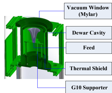
FIGURE 15. 3-D structure with mechanical design for Cryogenic
