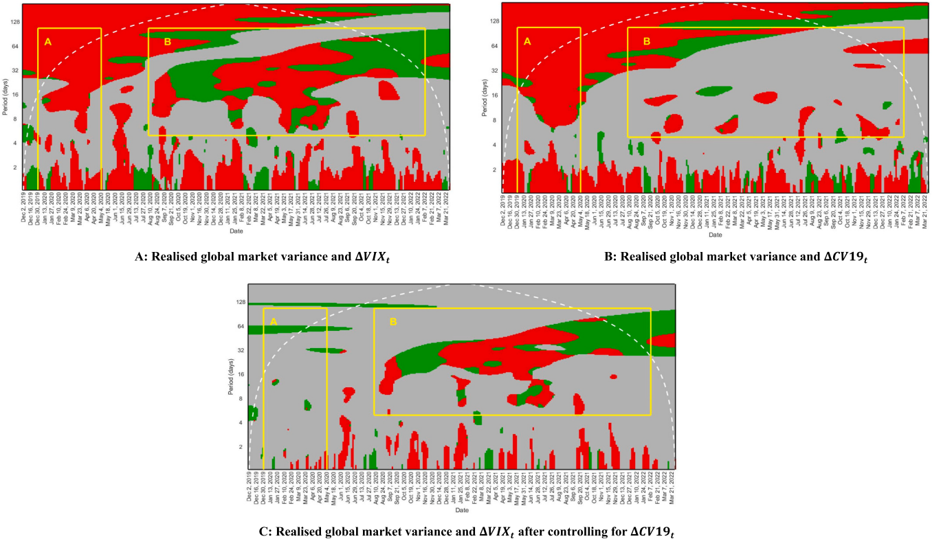
Fig. 4. Spectrograms for realised global market variance, V_{W,t}
