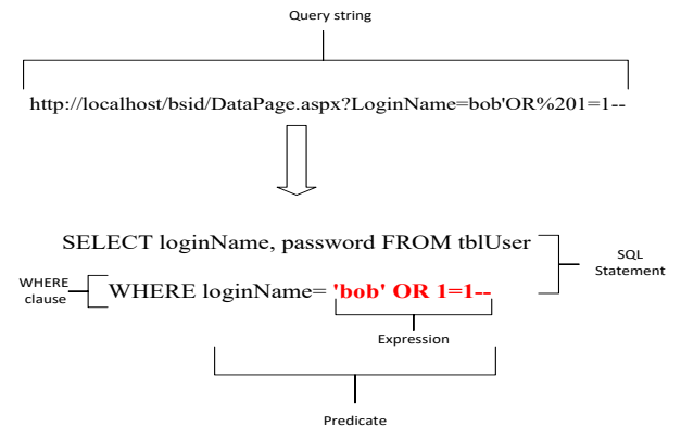
Fig. 1. Query string and SQL query element.
