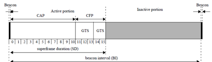
Fig. 1. IEEE 802.15.4 superframe structure
