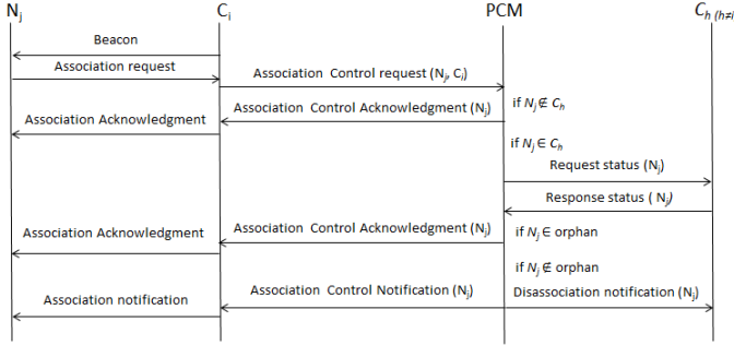
Fig. 4. Controlled Association process.
