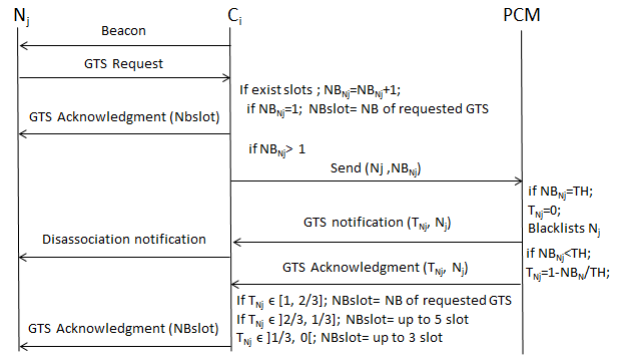
Fig. 5. Trust-based GTS Allocation process.
