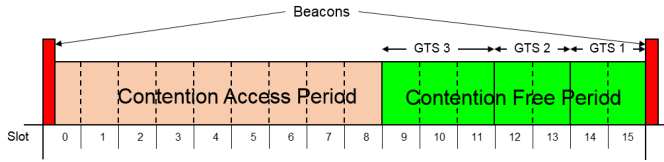
Fig. 2. Structure of the active periods with GTSs
