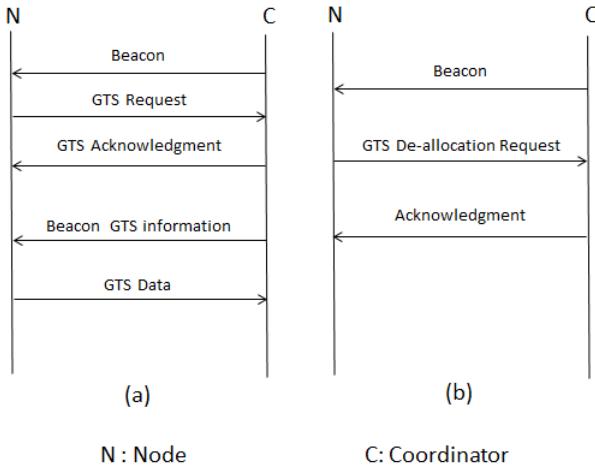
Fig. 3. (a) GTS allocation process, (b) GTS de-allocation processes.
