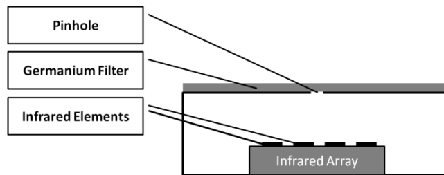
Fig. 2. Optical arrangement.
