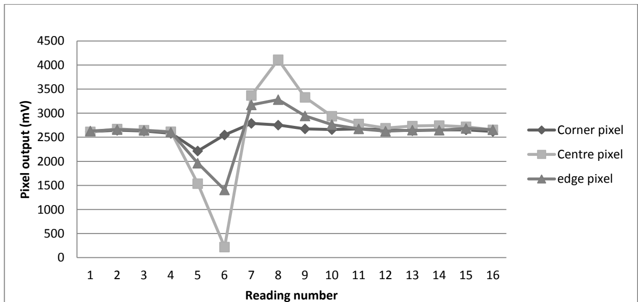
Fig. 6. Variations in pixel response
