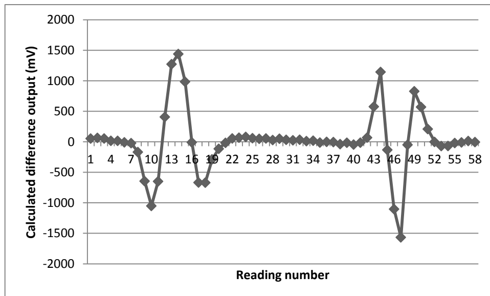
Fig. 7. Using the detector in differential mode to detect a hand swipe moving backwards and forwards across the detector.
