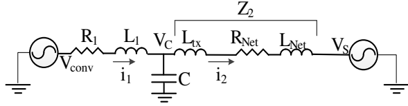
Figure 1. Schematic of VSC connected to power grid.
