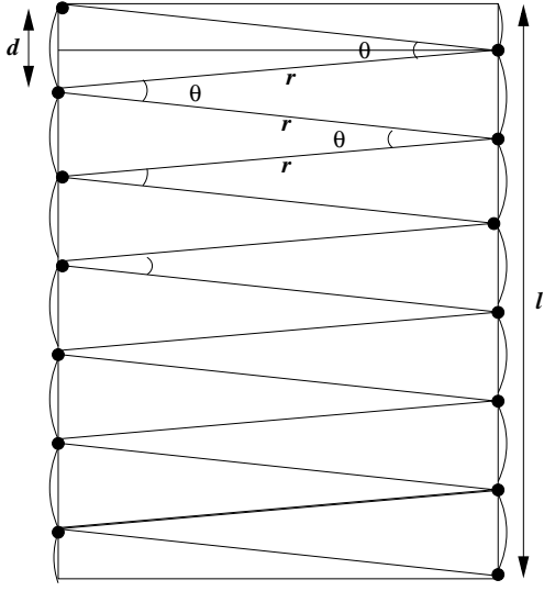
Figure 5: Coverage of depot using sectored sensing disc.
