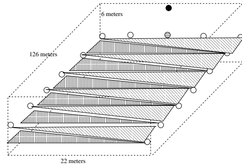
Figure 4: Sensing range of the sensors.
