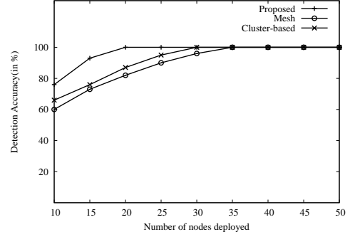
Figure 6: Detection Accuracy vs. Number of nodes deployed in the chain
