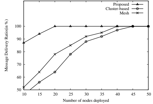
Figure 8: Message delivery ratio with food grain bins inside the depot.
