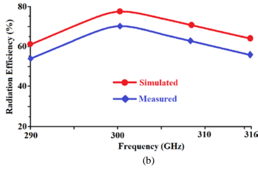
Fig. 6. (a) Gain, and (b) radiation efficiency as a function of frequency.
