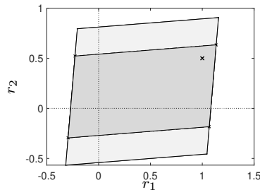
FIGURE 4.3. Feasible sets of reference vectors r = (r_1 \ r_2)^T for \phi_1 (darker grey) and \phi_2 (lighter grey) regions. The reference r in (4.8) is marked with a cross.
