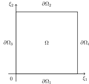
FIGURE 4.2. Square domain \Omega \subseteq \mathbb{R}^2 .
