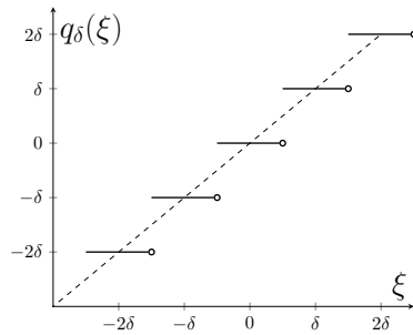
FIGURE 4.1. Quantization function q_\delta .
